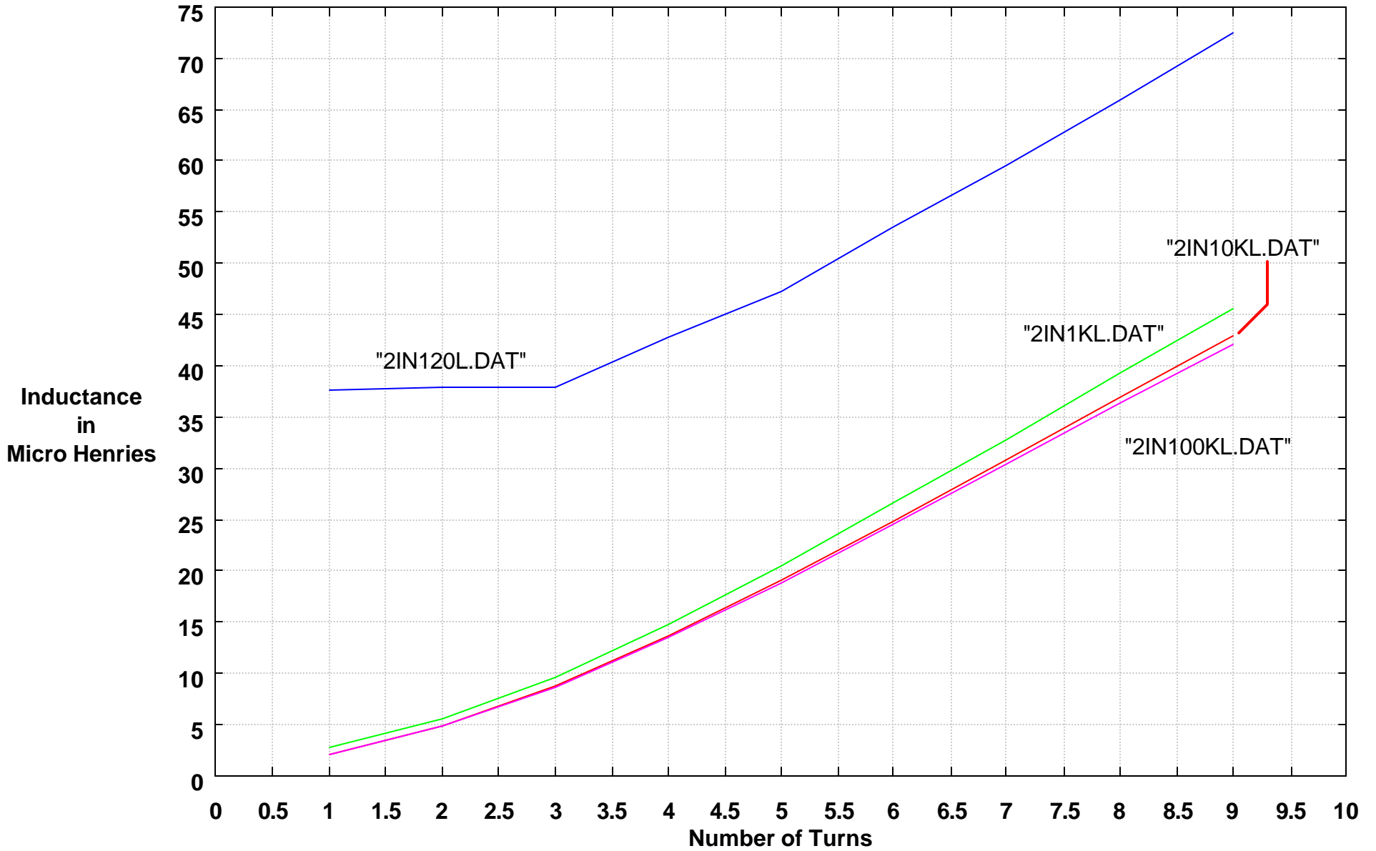
Measured Inductance of 2inch Flat Spiral Primary Using HP 4263B LCR Meter
